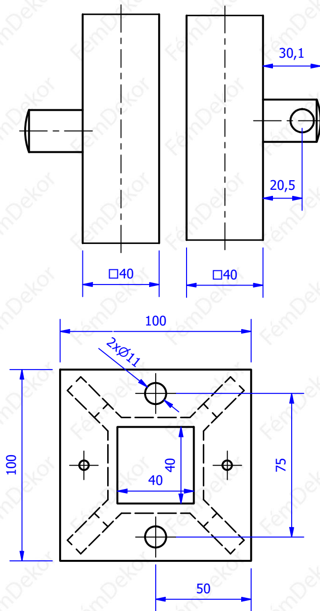
B (1:2) C (1:2)
